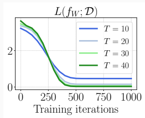
(a) Linear regression
