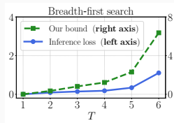
(a) Breadth-first search
