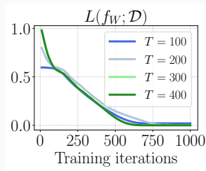
(b) Quadratic regression
