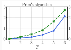
(c) Prim's algorithm
